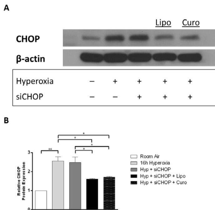
Figure 2. In vitro effect of Curosurf® as a transfection reagent on CHOP expression in hyperoxic exposure. (A) The protein expression of CHOP in MLE-12 cells was ascertained under the conditions described, with \beta -actin controls. (B) Corresponding relative CHOP protein expression in MLE-12 cells. Each bar represents the mean \pm the SEM for a minimum of 3 samples per group. * P \leq 0.05 , ** P \leq 0.01 , unpaired t -test. (Curo = Curosurf®, Hyp = hyperoxia, Lipo = Lipofectamine 2000®, siCHOP = CHOP siRNA)
